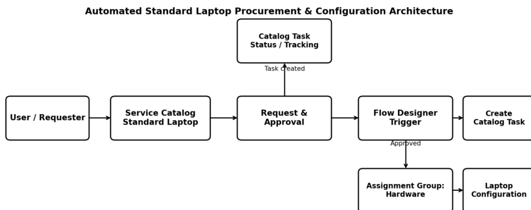
Figure 1: Architecture and data flow of the automated Standard Laptop procurement solution
